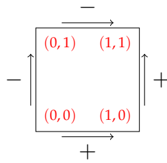
FIGURE 1. The boundary of the 2-cube consists of four 1-cubes (with the indicated parametrisations and signs)
