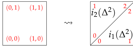
FIGURE 2. Subdividing a square into two triangles
